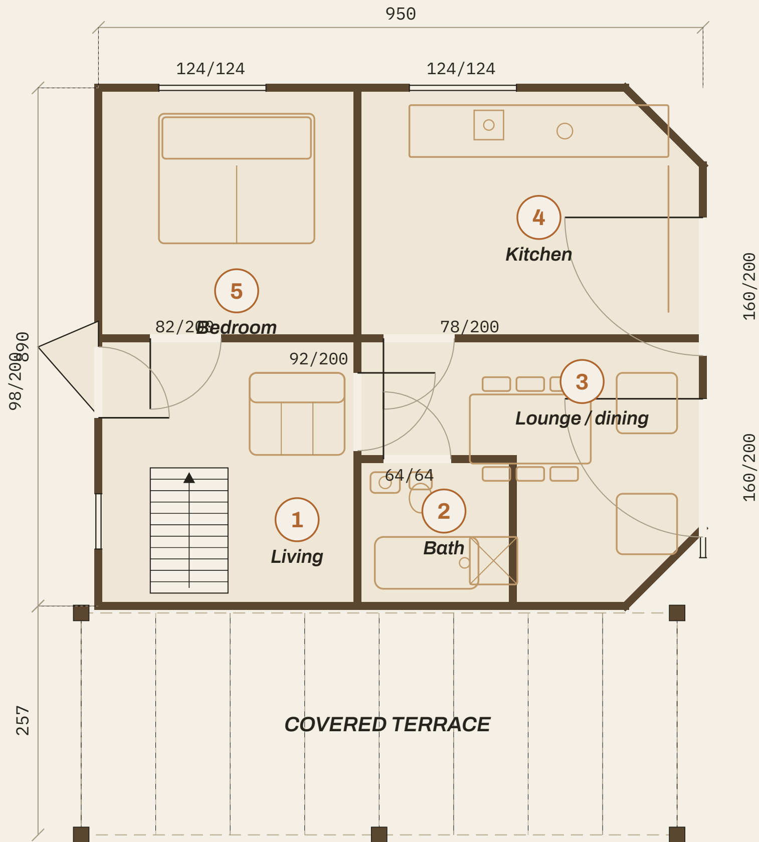
GROUND FLOOR · PARTER
